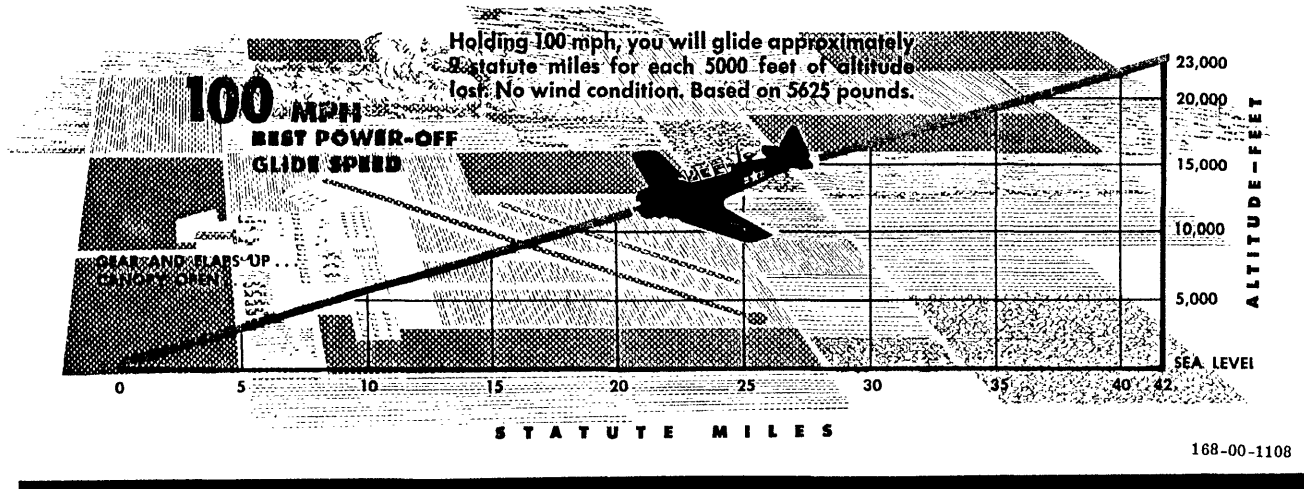
Figure 3-2. Maximum Glide
