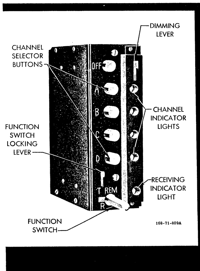
Figure 4-2. SCR-522A Radio Control Panel— Airplanes AF51-14359 Through -14683
