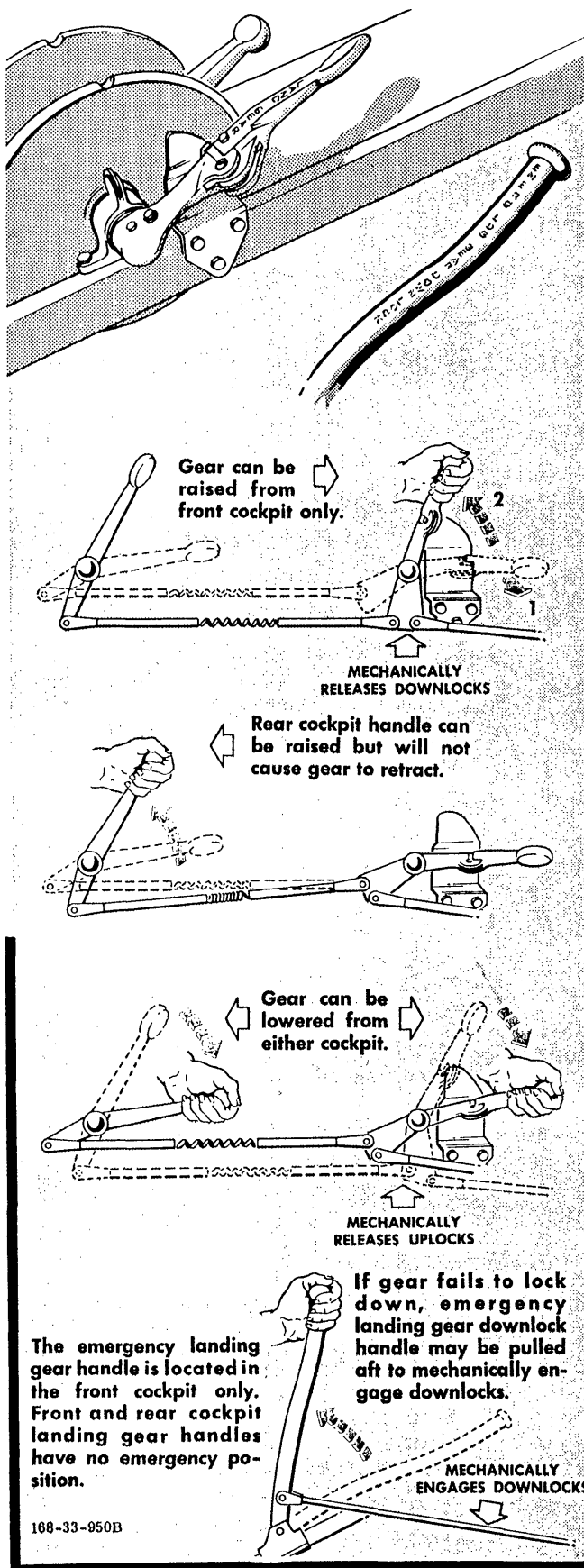
Figure 1-13. Landing Gear Handles and Emergency Downlock Handle
